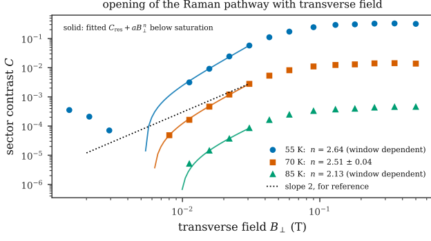
FIG. 4. Opening of the Raman pathway with transverse field, full Liouvillian. Solid curves are fits of C = C_{\text{res}} + aB_{\perp}^n over the pre-saturation range; the dotted line is a slope-2 reference. The fitted exponent is quoted only where it survives a change of upper cutoff (70 K); at the other temperatures the interval between the residual plateau and saturation is too narrow to determine it, and the legend says so.
