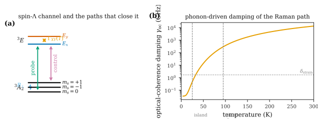
FIG. 1. (a) The NV - spin-A channel. Probe and control address two ground spin sublevels through the ^3E orbital doublet. Because the optical dipole is orbital, the two legs reach orthogonal spin states and the leading Raman vertex is closed at B_\perp = 0 ; a transverse field mixes the ground sublevels and opens it. Phonon-induced hopping \Gamma_{XY}(T) between the excited branches damps the pathway. (b) Optical-coherence damping \gamma_{oc}(T) over the range studied, with the transverse strain splitting marked for scale. The island boundaries found in Sec. III are indicated.
